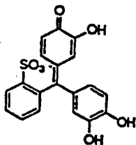
PYROCATECHOL VIOLET
